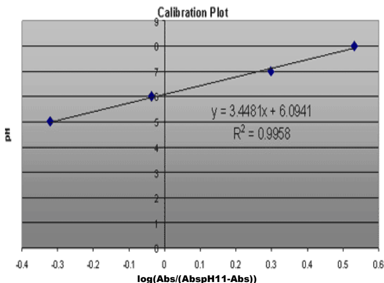
Figure 5. Calibration Plot
